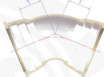
45° Double Socket Bend
